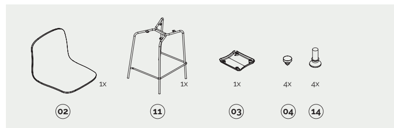
stool h.650 with variable inclination glides
